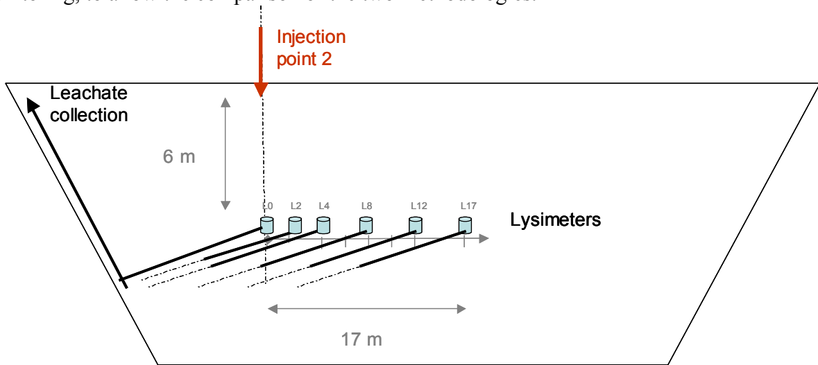
Figure 4. Plot of the lysimeter set-up (cluster B)
