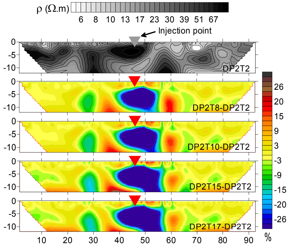
Figure 2. Preliminary ERT study of the plume of the recirculation system: Interpreted resistivity variations compared with an electrical imaging before the beginning of injection
