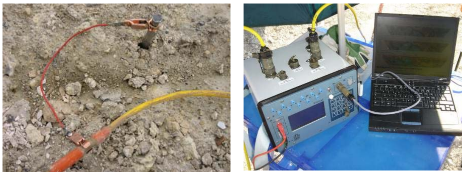
Figure 1. Experimental set-up of the ERT measurement
